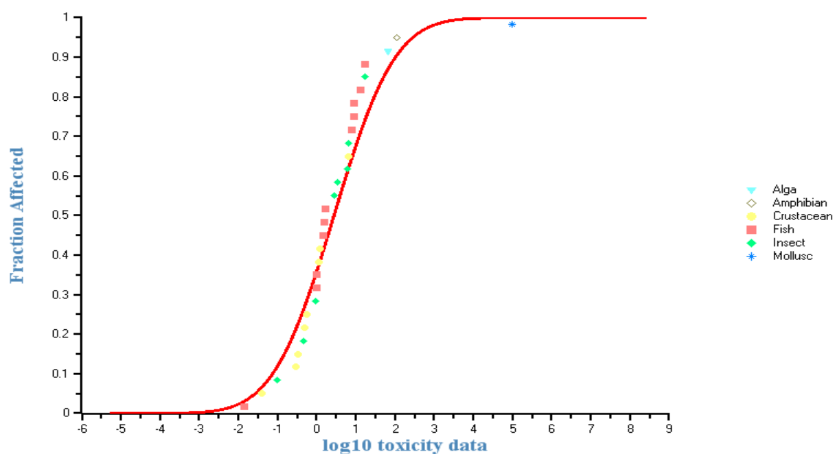
Figure 2.2 Cumulative distribution function of freshwater short-term data ( \mu\text{g l}^{-1} ) for permethrin
