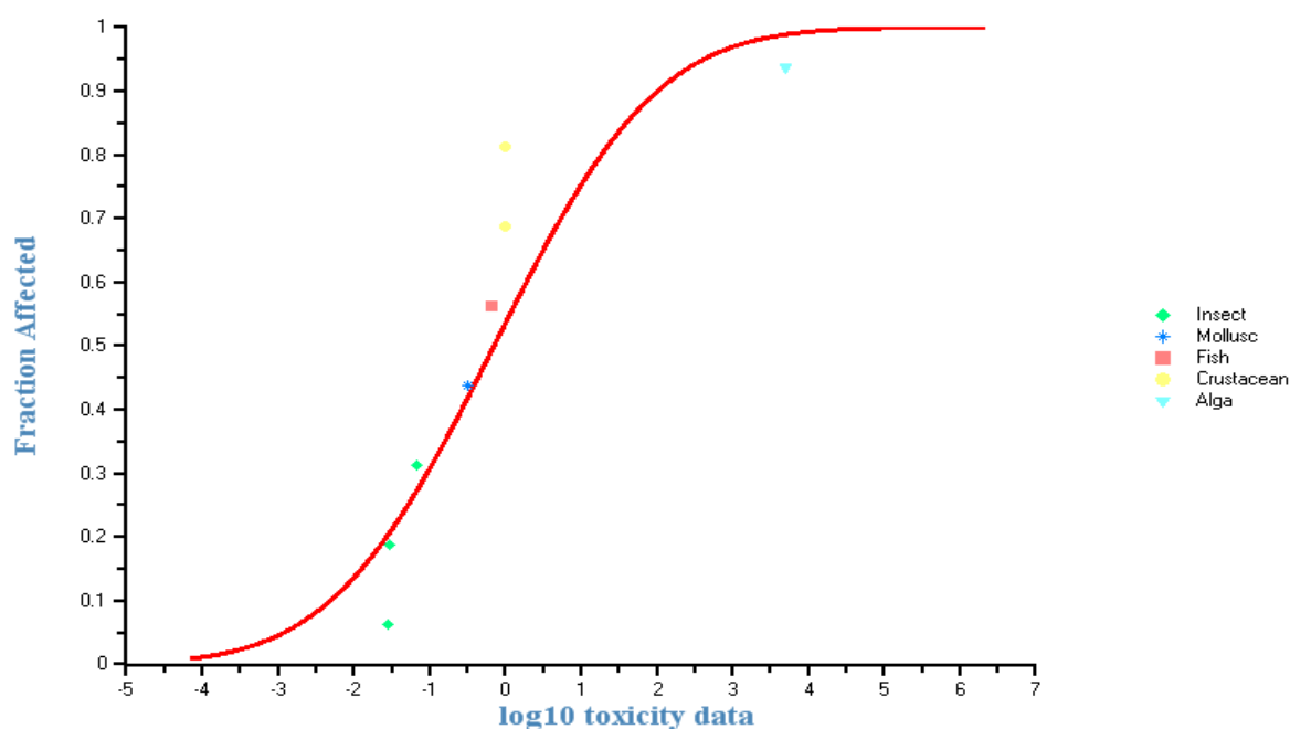
Figure 2.2 Cumulative distribution function of freshwater short-term data ( \mu\text{g l}^{-1} ) for permethrin
